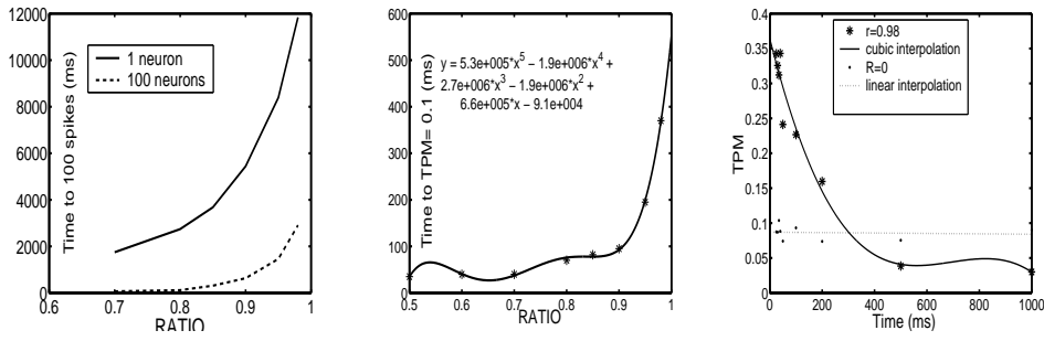
Fig. 2. Coherence = 15%. Left: Time to get a hundred spikes versus r , with a population of a hundred neurons and with a single neuron. Middle: Illustration of the numerical estimation of the time to reach an acceptable discrimination performance ( TPM = 0.1 ). Right: Comparison of the evolution of the TPM for long time windows, reaching to one second, with r = 0.98 and r = 0 . When we wait for one second, the TPM for r = 0.98 is 0.03 and the TPM for r = 0 is 0.09
